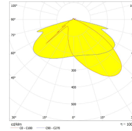
Luminance Distribution
