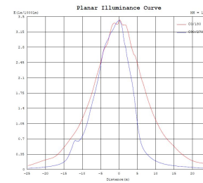
Illumination Curve
