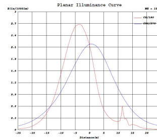
Illumination Curve
